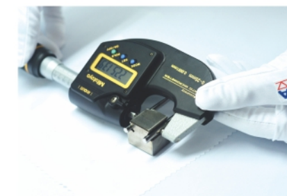
測量溝槽 Measure Groove
